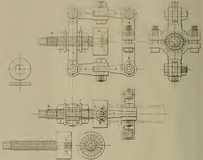
DETAILS OF HAND MILLER FOR SUPERHEATER UNITS
